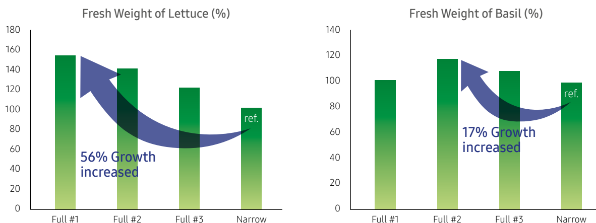
Figure 4. Performance of narrow and full LED spectrum
